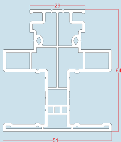
MULLION 70-002
